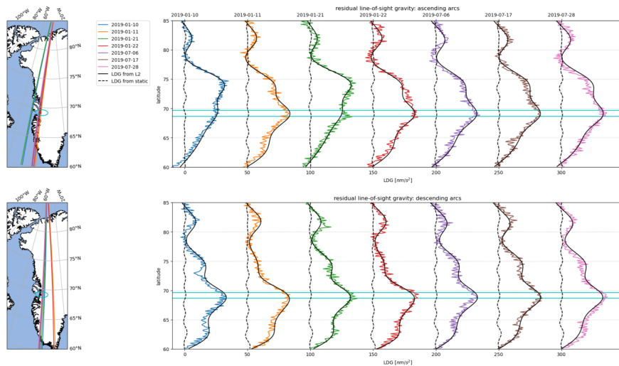
Figure 1: This figure is the main result and shows the residual line-of-sight gravity (LGD) from laser ranging (LRI) and the monthly gravity field from JPL (L2) for four days in January 2019 and three days in July 2019.
