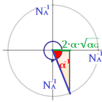
Figure 7. The angle in a^{-1} radians.
