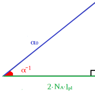
Figure 13. Geometric representation of the relationship between the Bohr radius and the Planck length.
