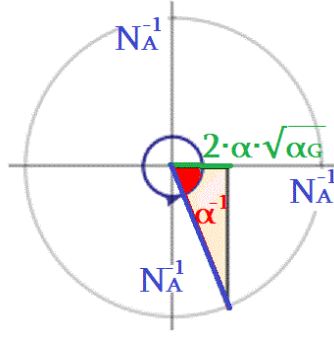
Figure 14. The angle in \sigma^{-1} radians.
