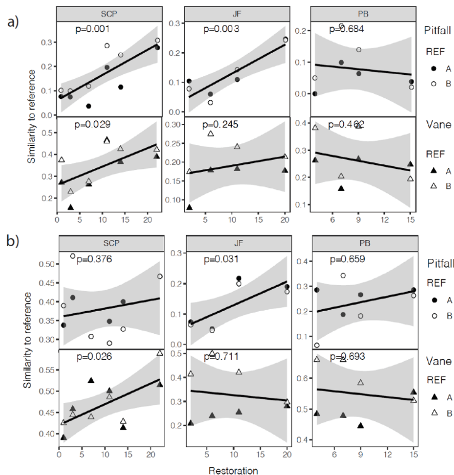
Figure Similarity (Bray-Curtis) of restoration sites of different ages (years) to communities in both reference sites. a) Shows the invertebrate communities and b) the results of the plant assay. Lines indicate linear models with 95% confidence interval shown with shading. P-values for the linear models shown for each plot. Removing the two extra sites in the SCP (7,11 years) did not change the relationships or the significance of the models. SCP-Swan Coastal Plain, JF-Jarrah Forest, PB-Pilbara.
