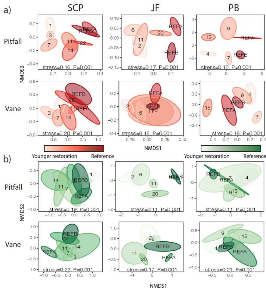
Figure NMDS ordinations of Invertebrate and plant communities in restoration and reference sites. Ellipses were drawn using ‘Ordellipse’ in the vegan R package and indicate 95% confidence interval of the group. Stress values and significance of PERMANOVA tests indicated in the bottom of each facet. SCP-Swan Coastal Plain, JF-Jarrah Forest, PB-Pilbara.
