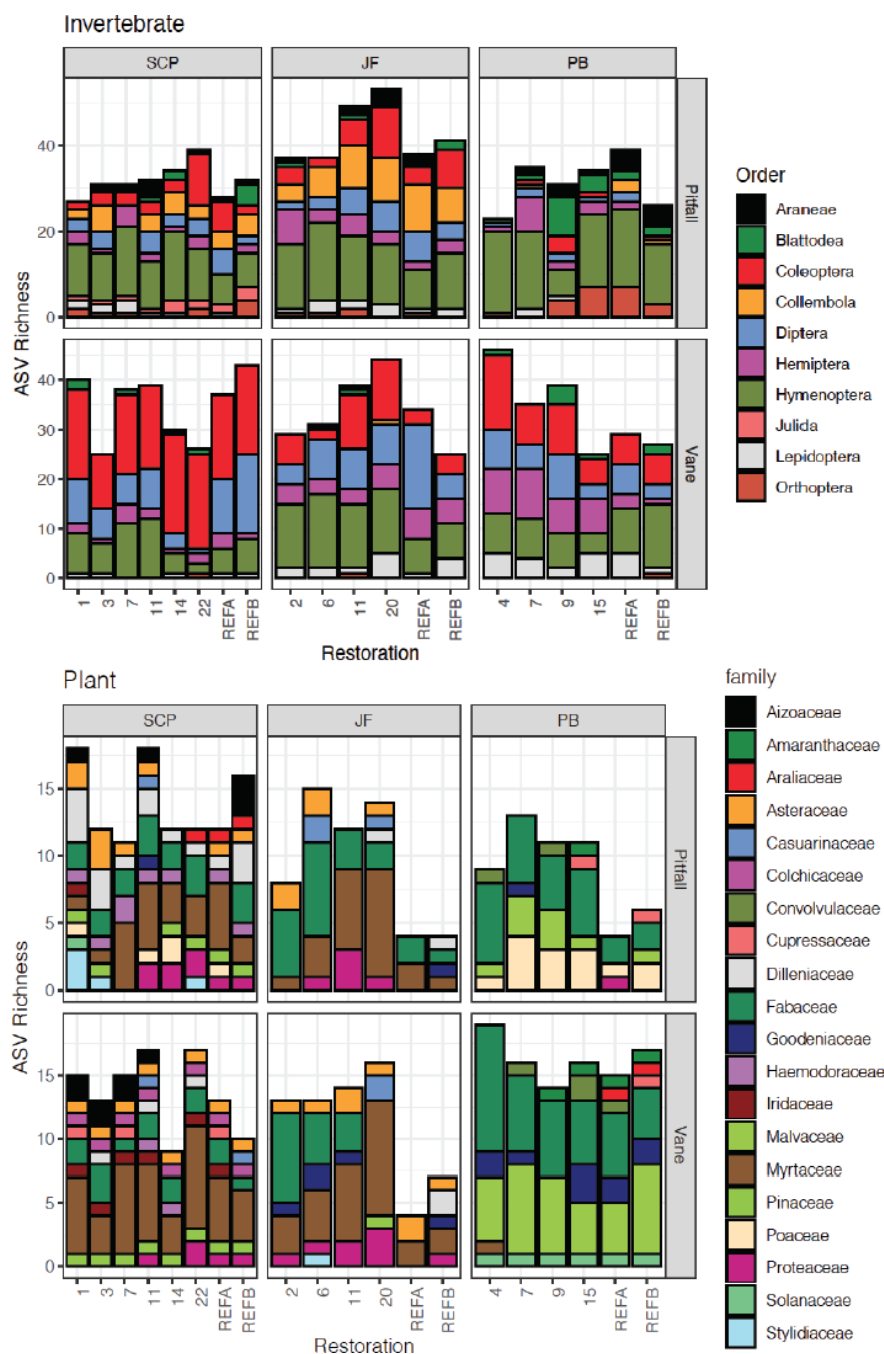
Figure Composition of invertebrates (above) and plant (below) communities detected from pitfall and vane traps. Shows the number of ASVs in each order (invertebrates) or family (plants) at all restoration and reference sites. SCP-Swan Coastal Plain, JF-Jarrah Forest, PB-Pilbara.
