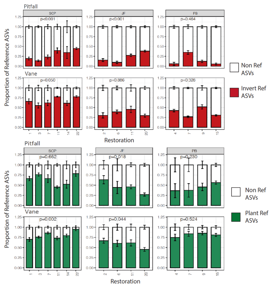
Figure Proportion of reference associated ASVs in the different sites, separated into a) invertebrate and b) plant communities. P-values indicate the significance of the relationship between the proportion of reference ASVs and age of restoration (years). SCP-Swan Coastal Plain, JF-Jarrah Forest, PB-Pilbara.
