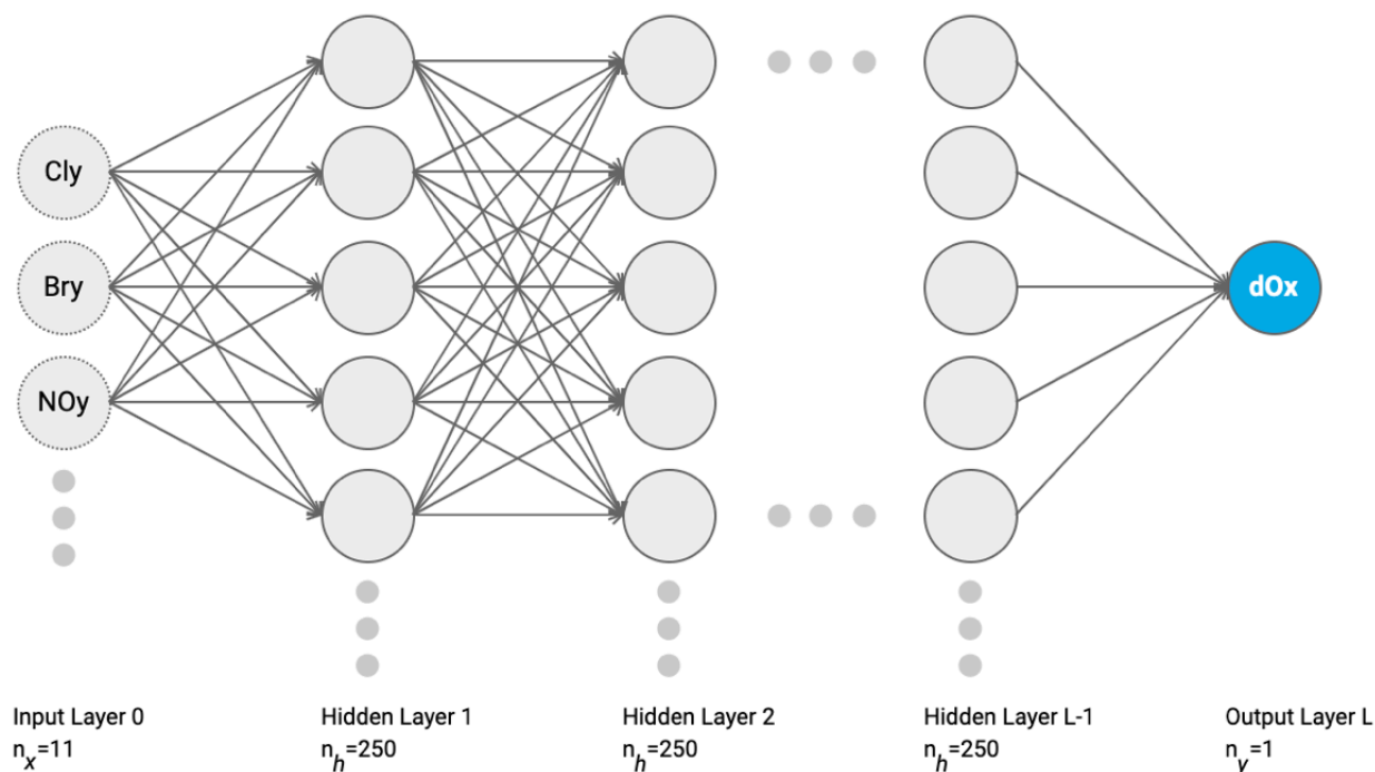
Fig. 3: Sketch of the NN-architecture. A fully connected NN is shown. On the left side the input neurons are shown, followed by the hidden layers (middle) and the regression output neuron to the right. The number of layers and the number of neurons per layer need to be optimized by a hyperparameter search.
