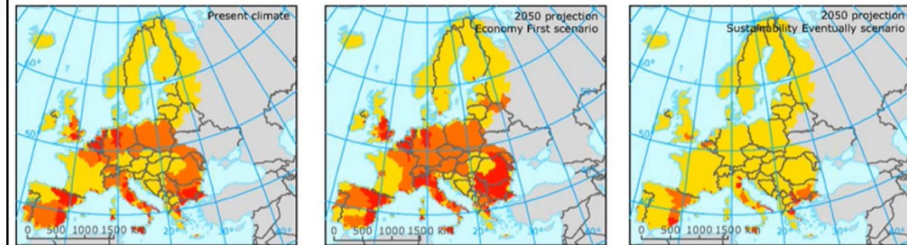
Annual water stress for present conditions and projections for two scenarios
